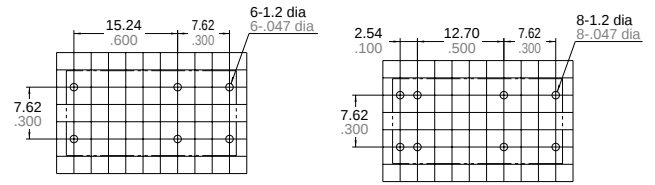
PC board pattern (Bottom view) Single side stable 1 coil latching type
