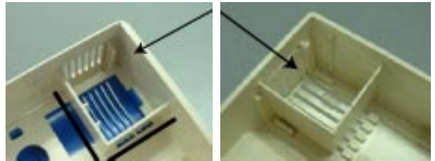
Fig. 19-1 - Example of sensor compartment in detector housing
