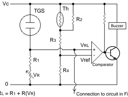
Fig. 14 - Conventional circuit for temperature compensation
