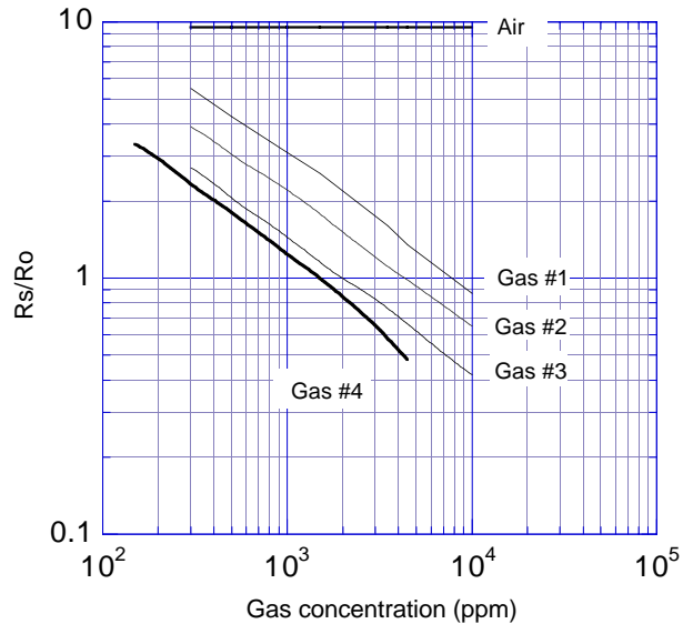
Fig. 5 - Typical sensitivity characteristics
