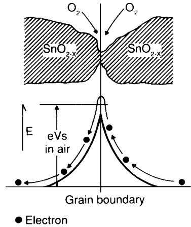
Fig. 1 - Model of inter-grain potential barrier (in the absence of gases)
