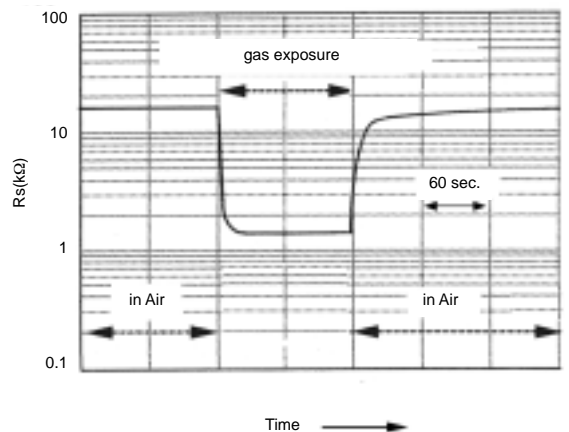
Fig. 6 - Typical sensor response
