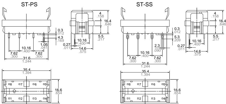
ST-SS Solder terminal socket
